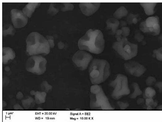
Figure 6. Photo, made by the scanning electron microscope (SEM), of microspheres in proportion losartan potassium : Eudragit L30D55 1 : 3 with addition of triethyl citrate in amount of 10% of dry matter drug : polymer ( sample W3 magnification 10000×)
