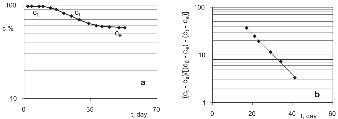
Figure 3a. Diagram presenting changes in concentration of ATO in following conditions: a humid atmosphere (RH = 76.4%) at temp. 363 K; where C_0 - initial concentration of ATO at time t_0 , C_t and C_e concentration of ATO at time t and t_e , respectively. Figure 3b. Semilogarithmic plot (C_t - C_e) / [(C_0 - C_e) - (C_t - C_e)] = f(t) for degradation of ATO in solid phase (RH = 76.4%; temp. 363 K).
